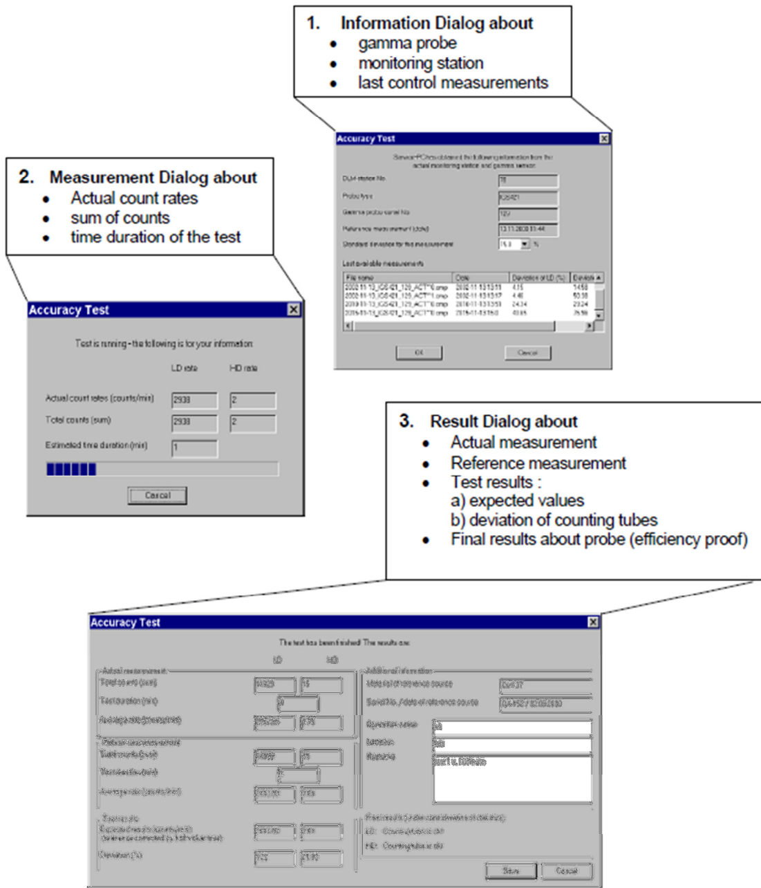
Figure 2: User Dialogues of Accuracy Test Procedure
